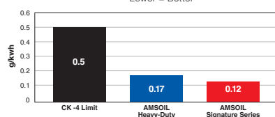
OIL CONSUMPTION Lower = Better
