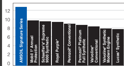
ACID NEUTRALIZING POWER Represented By Total Base Number (TBN) in ASTM D2896
