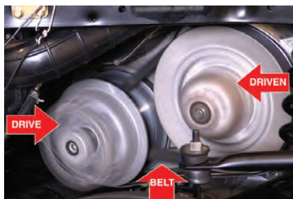
CVTs use variable-diameter pulleys to create the optimum gear ratio depending on conditions.
