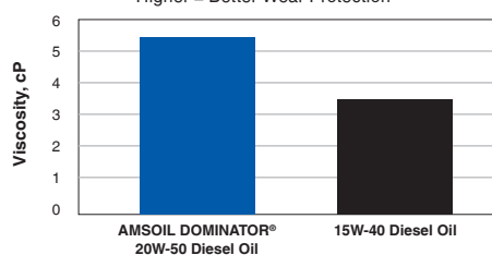
HIGH-TEMPERATURE/HIGH-SHEAR (HTHS) VISCOSITY Higher = Better Wear Protection
