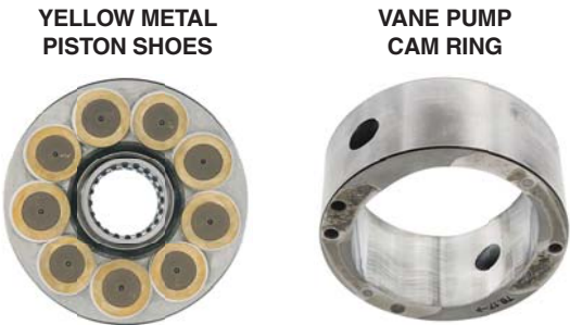
After 608 hours of strenuous pump testing in a Parker Hannifin (Denison) T6H20C Hybrid pump, the piston shoes demonstrated only moderate polishing and trace, random scratches, proving AMSOIL Synthetic Multi-Viscosity Hydraulic Oil excels at protecting yellow metals. The vane pump cam ring exhibited only light polishing and trace scratching, further confirming the excellent wear protection provided by the oil.
