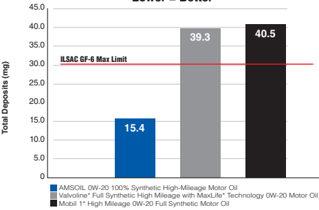
TEOST 33C (ASTM D6335) Lower = Better
