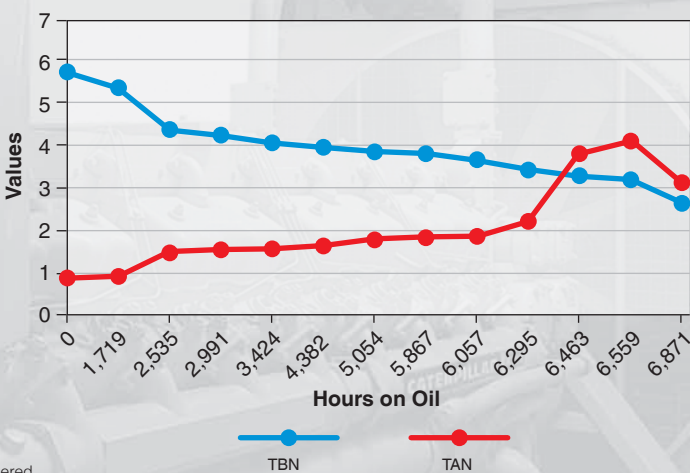
Total Acid & Base Numbers (ASTM D2896 & 664)
